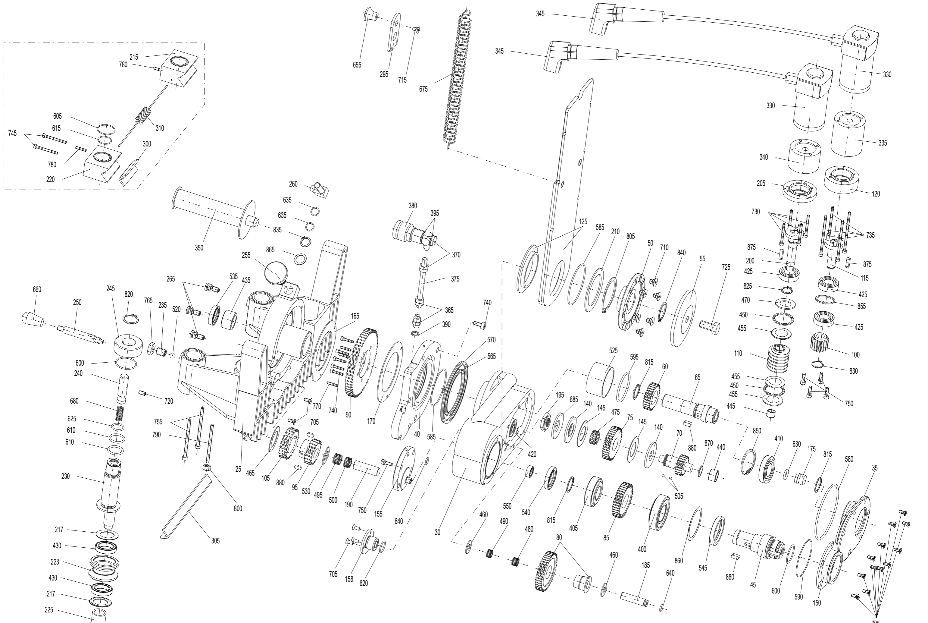
Diamond Wall Saw WS 75 Carriage WS 7520
